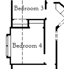
Optional Bedroom 4 with Box-Out Window (# 1303)
